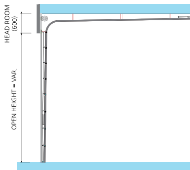
STANDARD TYPE
