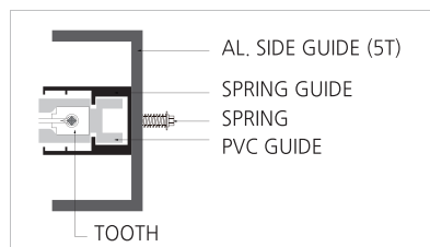
Guide Rail
